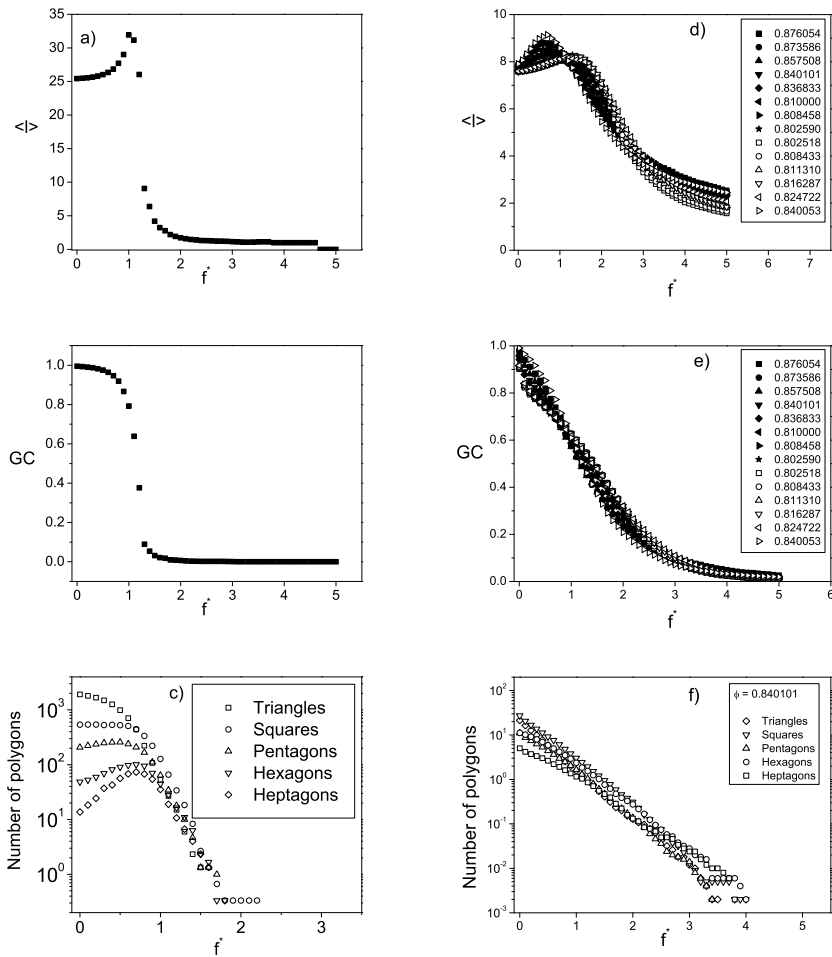
Figure 5. Average topological distance \langle l \rangle , giant component GC and populations of polygons for compressed, jammed networks (left) at \phi = 0.85 and tapped networks (right).
