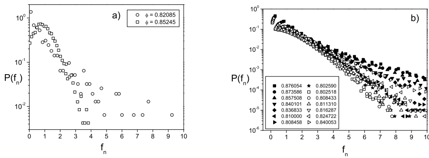
Figure 6. Normalized histogram of the normal contact forces for all the contacts. The variable f_n = F_n / \langle F_n \rangle is the normal contact force normalized by the average. a) Results for a compressed system before ( \phi = 0.82 ) and after jamming ( \phi = 0.85 ). b) Results for the packing states reached by tapping. Note that the values of packing fraction are shown in the caption in order of increasing \Gamma .
