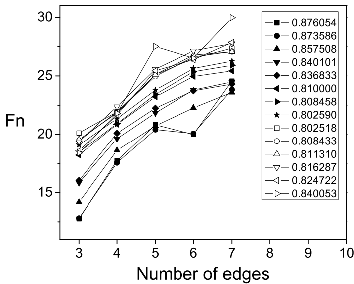
Figure 7. Normal force averaged over all the contacts of the polygons versus the size of the polygons. As in previous figures, the values of packing fraction are shown in the caption in order of increasing \Gamma .
