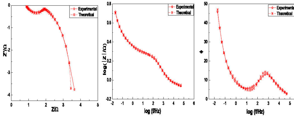
Fig. 9 – Theoretical and experimental impedance diagrams for electrode NiCoE.
