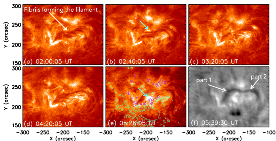
Figure 5 Formation of a long filament by the merging of fibril arcades to the N and W of the main sunspot in AR 12740 observed in AIA 304 (panels a–e) on 9 May 2019. Flux cancellation occurred in site a around 02:40 UT and continue (see arrows in panels a and b and the discussion in the text); this favoured the formation of a long curved structure. See text for the description of the evolution of this structure and the appearance of minor brightenings. A movie extending from 01:00 UT to 07:00 UT on 9 May accompanies this figure and Figure 6 (AIA304_09May2019_Fig3_Fig6.mp4). HMI contours of \pm 100 Gauss ( magenta/green for positive/negative polarities) are overlaid in panel e. Panel f presents H \alpha observations of the filament one minute before flare onset; its two parts are labelled as part 1 and part 2 and are indicated with white arrows (see text).
